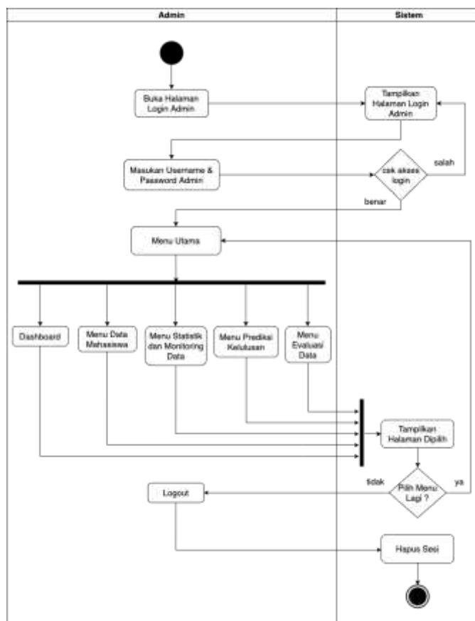
Gambar V. Activity Diagram Sistem
